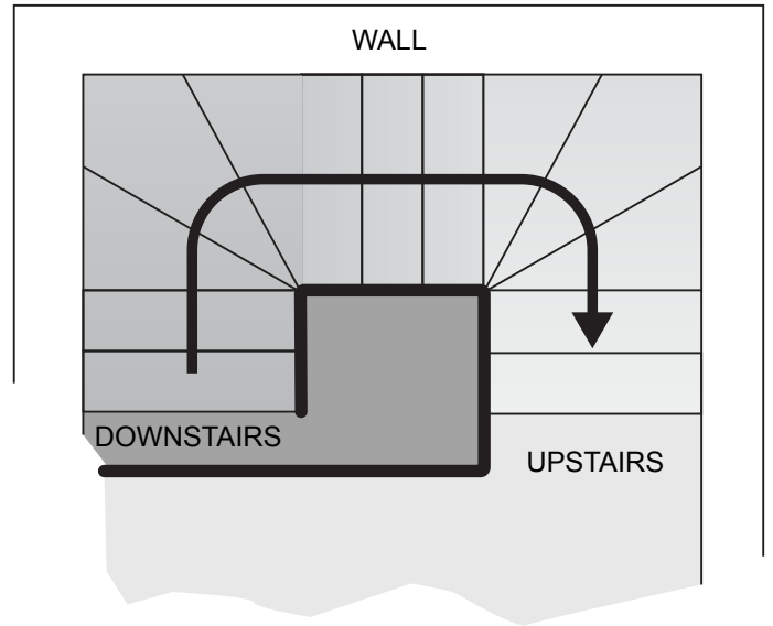
CURVED STAIRS with two winding bends
